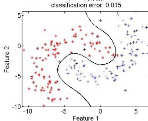
Nonlinear Models
